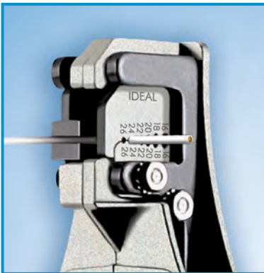
Gripper pads hold the wire securely in a centerline relationship with the blade.
